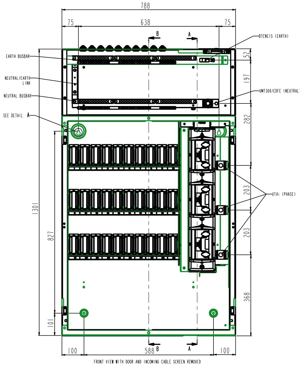
FRONT VIEW WITH DOOR AND INCOMING CABLE SCREEN REMOVED
