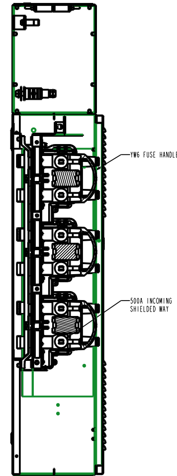
SECTION A-A SHOWING 500A INCOMING SHIELDED FUSEWAY
