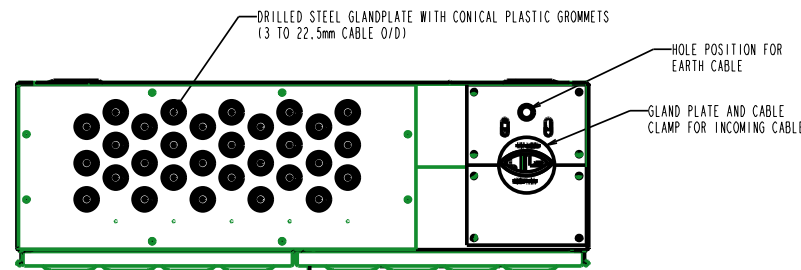
FRONT VIEW WITH DOOR AND INCOMING CABLE SCREEN REMOVED
